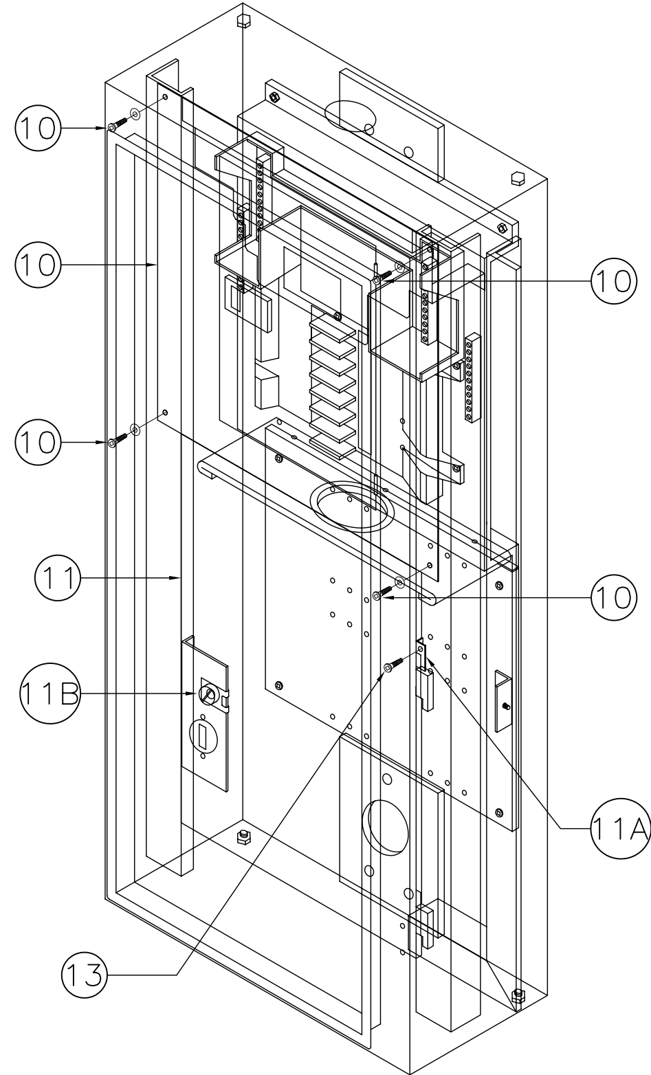
ASSEMBLY VIEW
