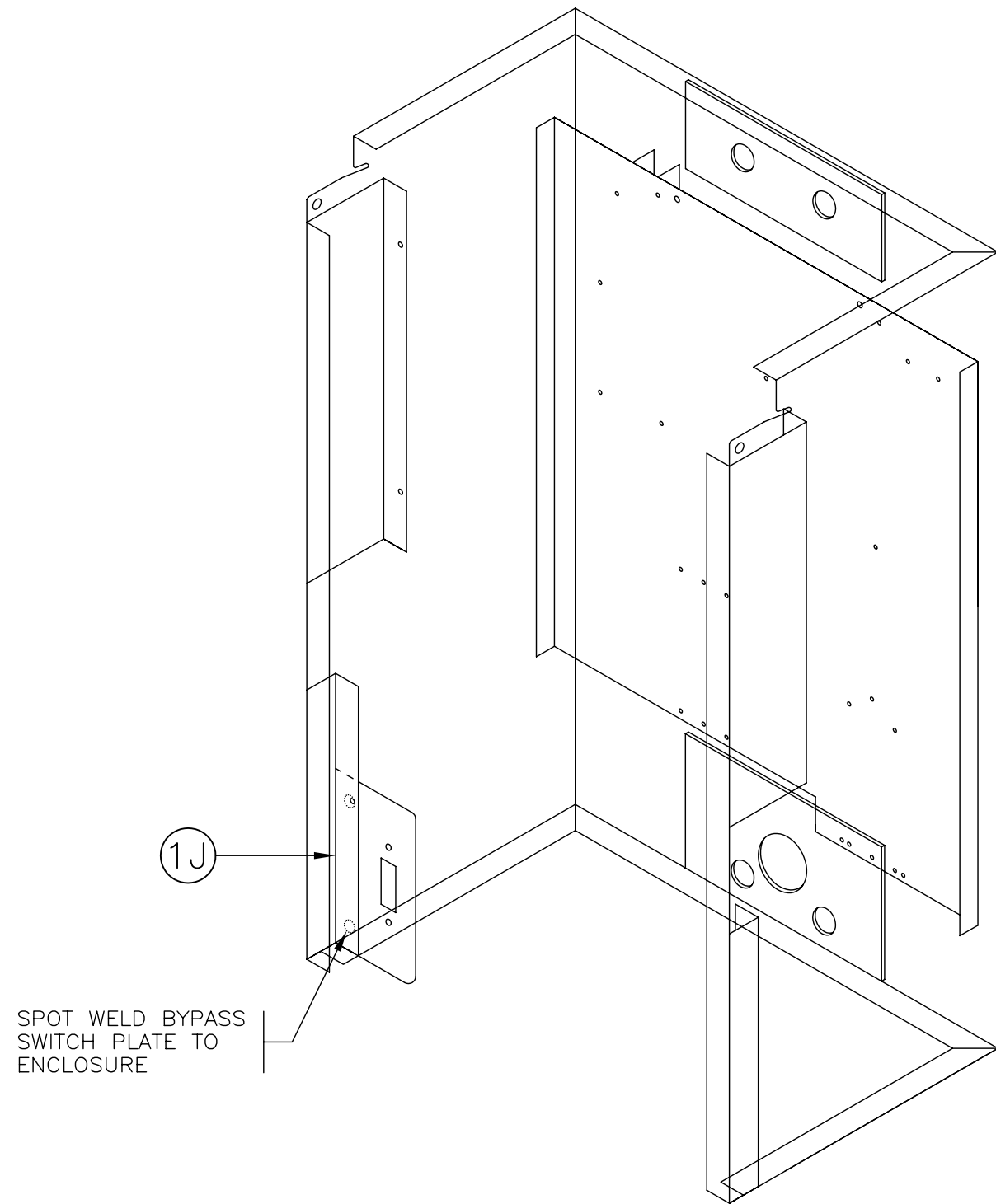
ASSEMBLY VIEW
