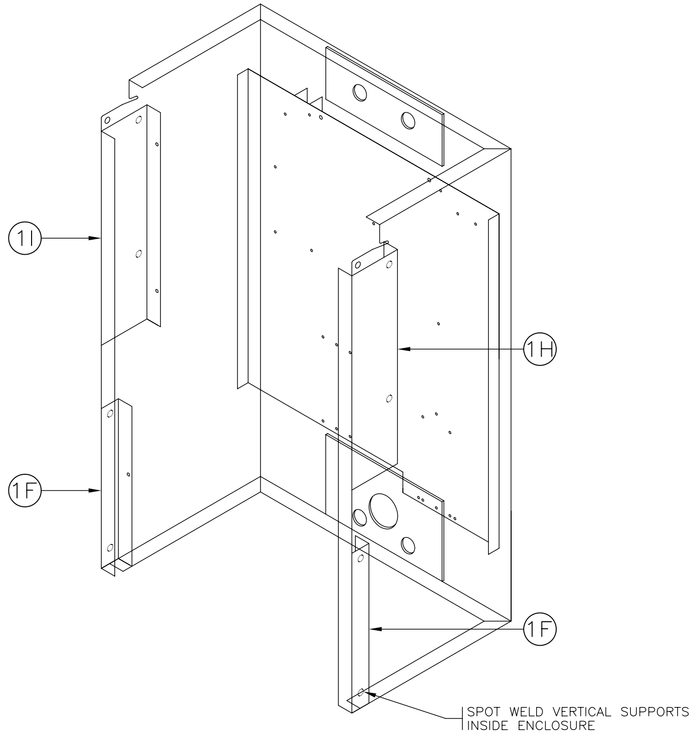
ASSEMBLY VIEW
