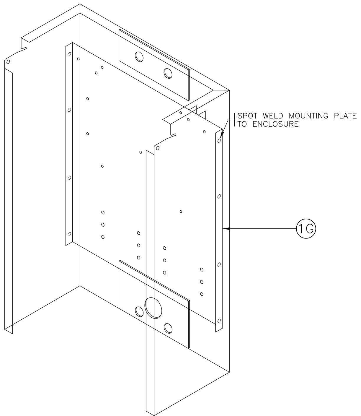
ASSEMBLY VIEW
