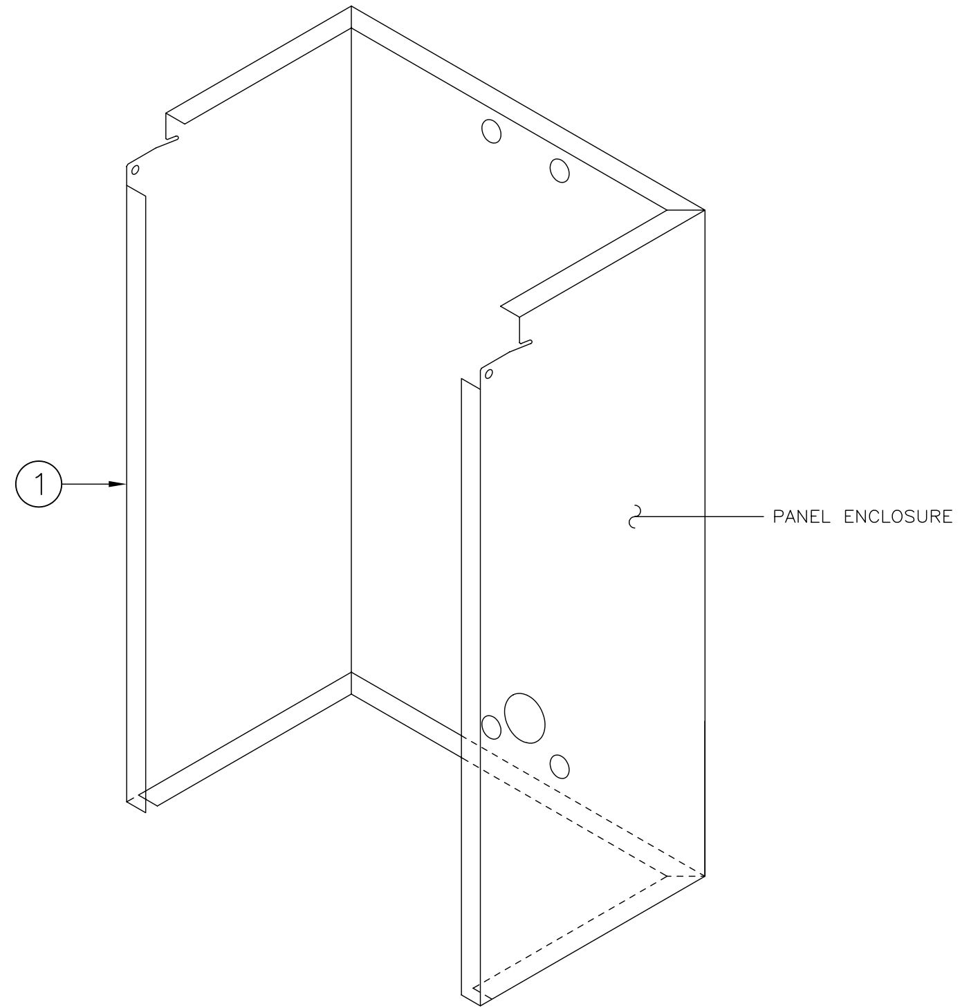
ASSEMBLY VIEW
