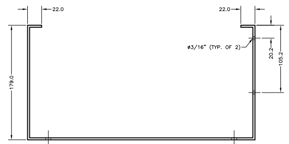
DETAIL C MATERIAL: 1/8" ALUMINIUM SCALE 1:5
