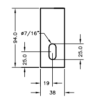
DETAIL D MATERIAL: 1/4" ALUMINIUM SCALE 1:5
