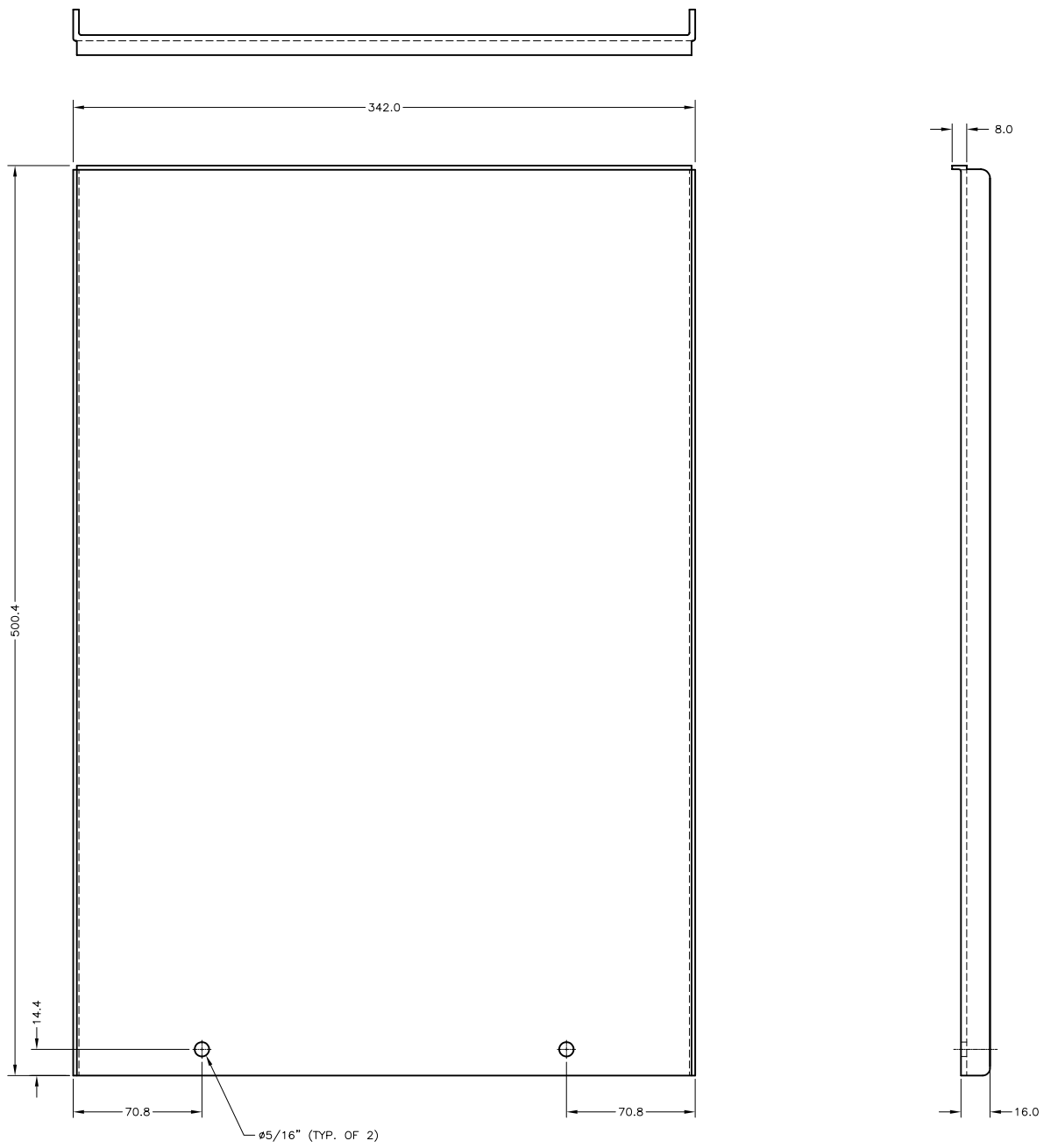
PART 002: JUNCTION BOX COVER MATERIAL: 1/8" ALUMINIUM SCALE 1:4
