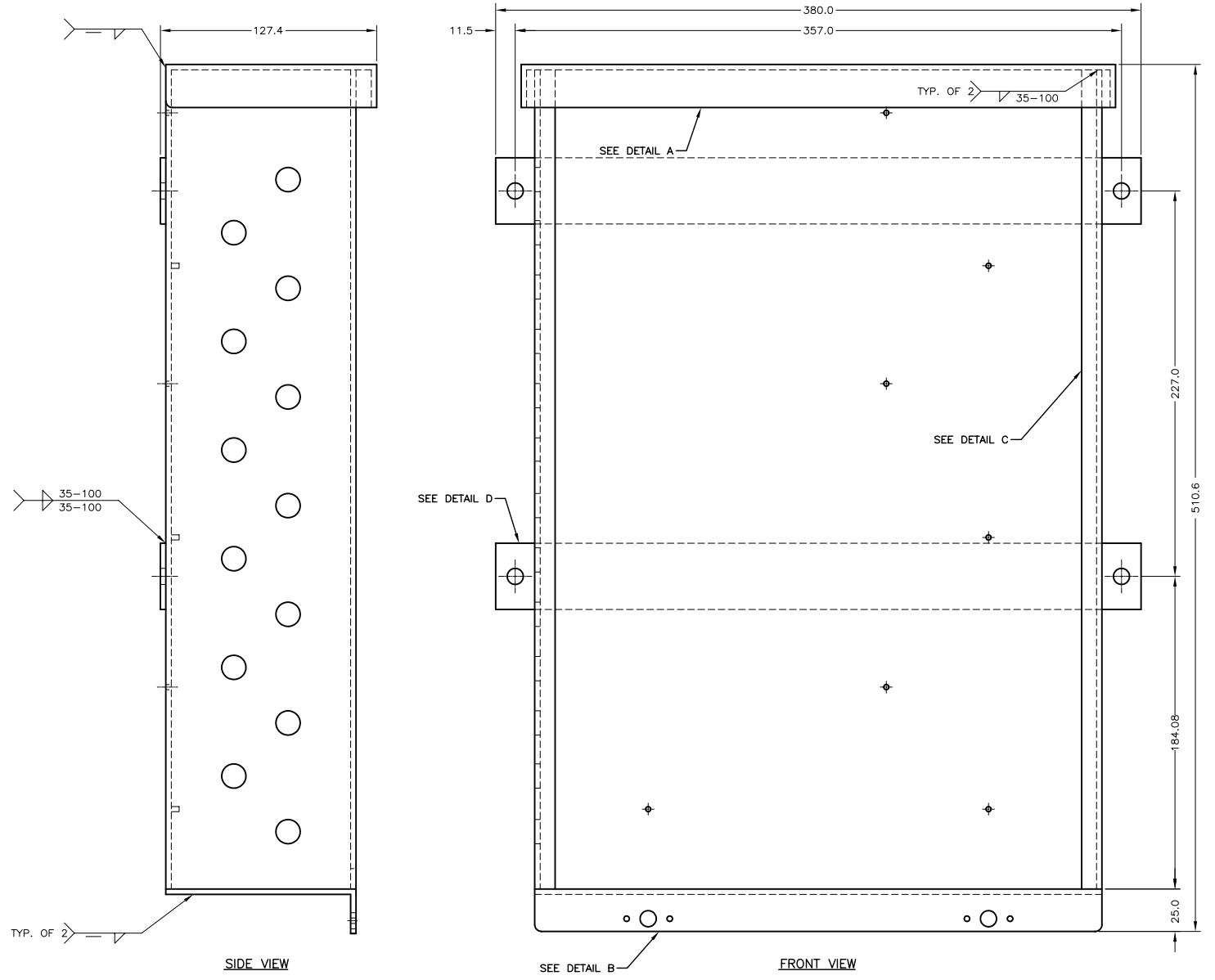
PART 001: JUNCTION BOX MATERIAL: 1/8" ALUMINIUM SCALE 1:4
