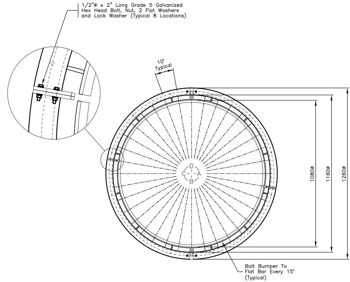
HIGHMAST RING Overall Dimensions
