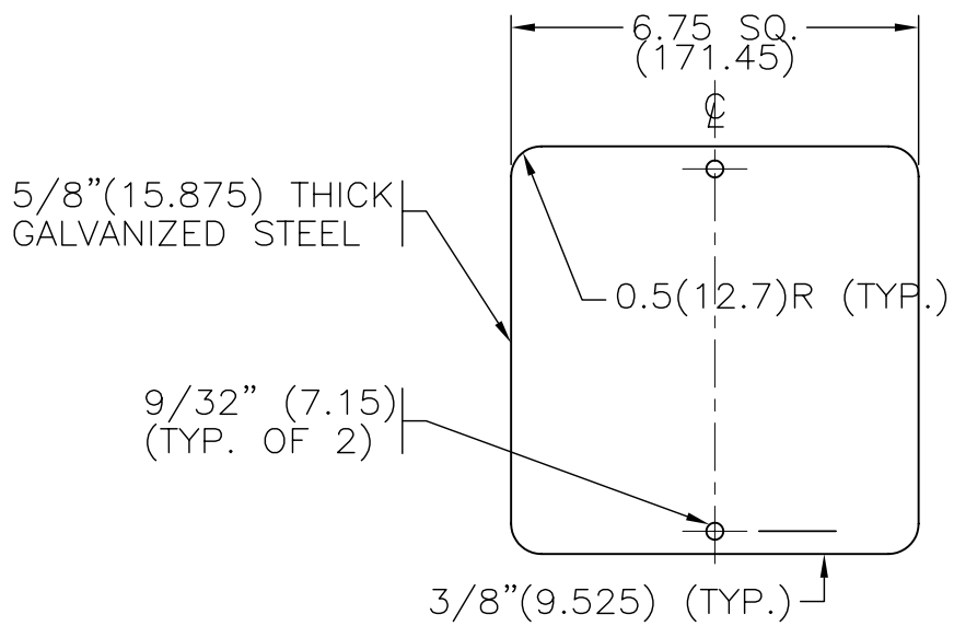
HANDHOLE COVER DETAIL (1 REQUIRED)
