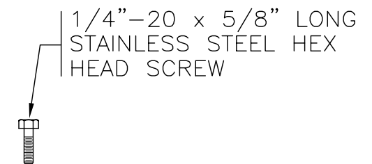
HANDHOLE COVER SCREW DETAIL (2 REQUIRED)
