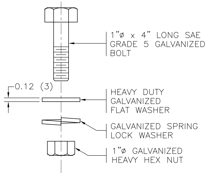
BOLT DETAIL (4 REQUIRED)
