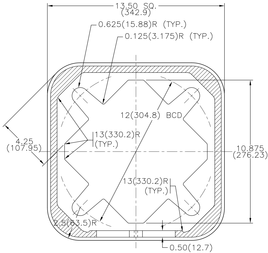
SECTION A
