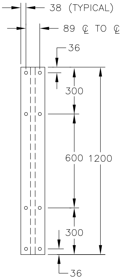
1200 COLUMN SN2171 (47 kg)
