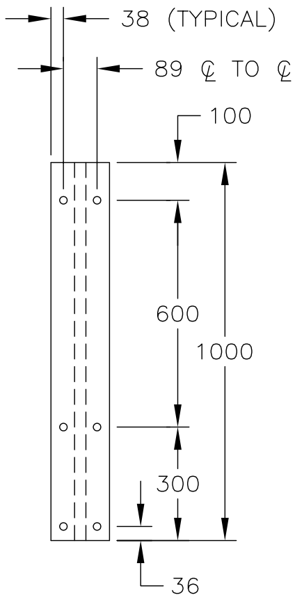
1000 COLUMN SN2170 (39 kg)
