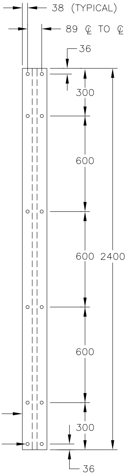
2400 COLUMN SN2173 (94 kg)
