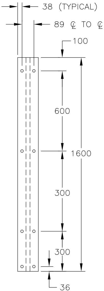
1600 COLUMN SN2172 (63 kg)
