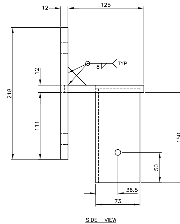
SIGN FRAME MOUNTED PIVOT ASSEMBLY
