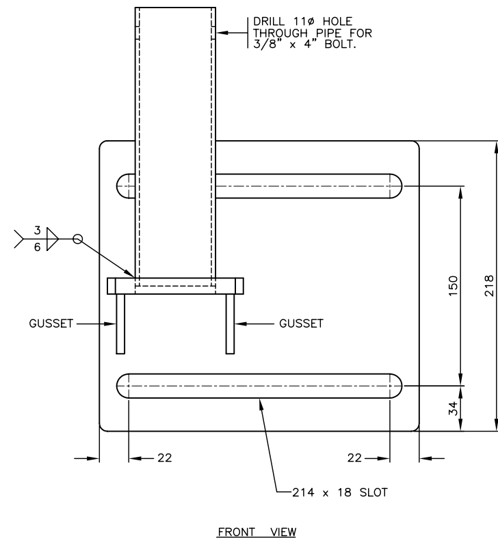
CLAMP MOUNTED PIVOT ASSEMBLY
