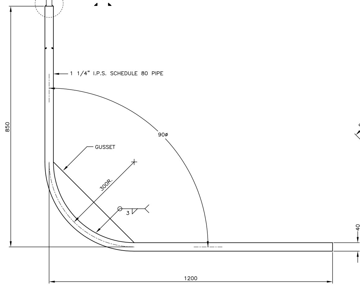
SIGN LUMINAIRE PIPE BRACKET (ITEM D)
