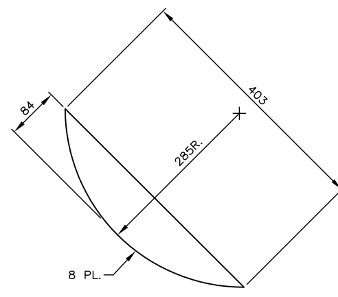
GUSSET PART OF ITEM D
