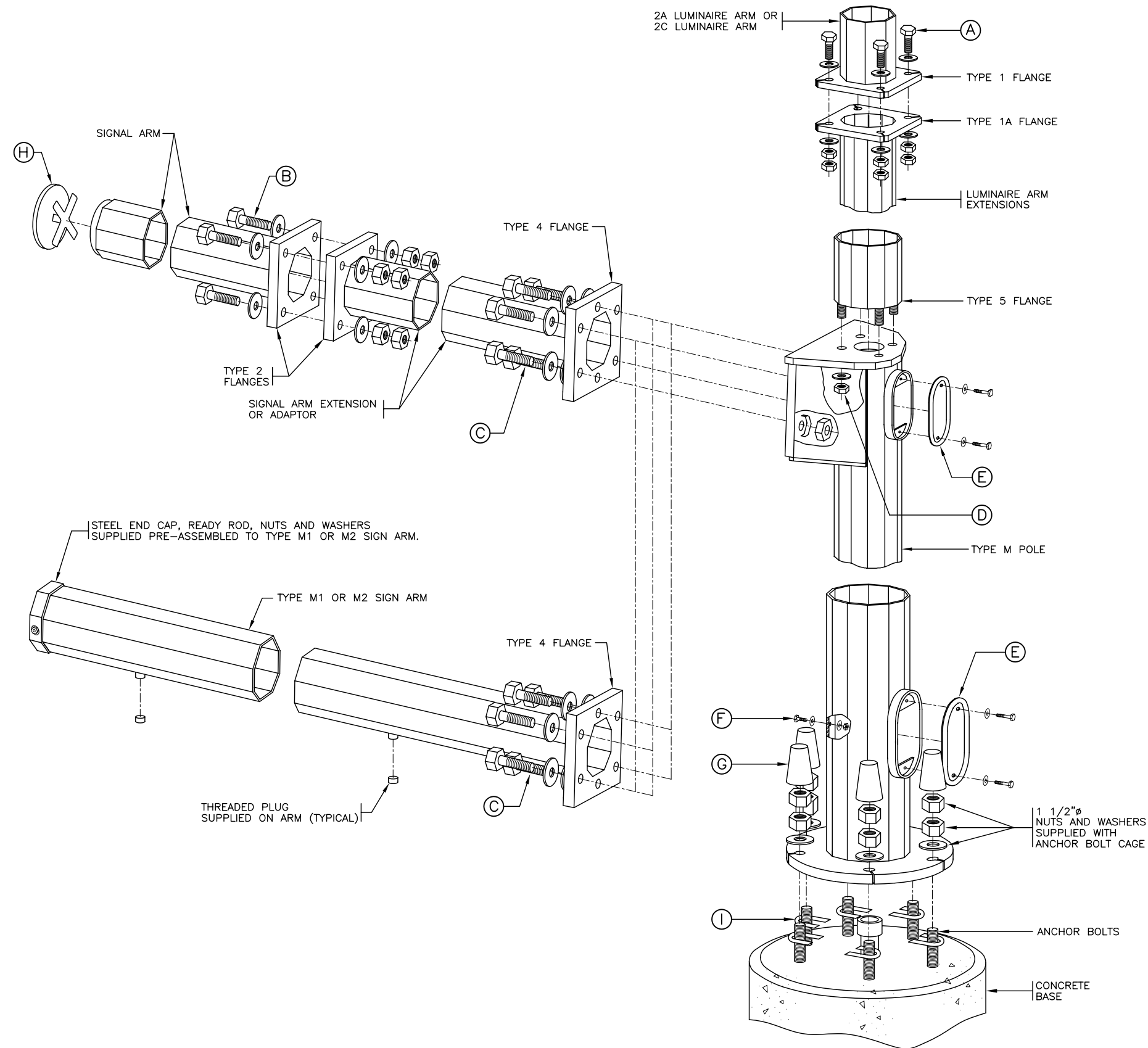
POLE ASSEMBLY DETAIL
