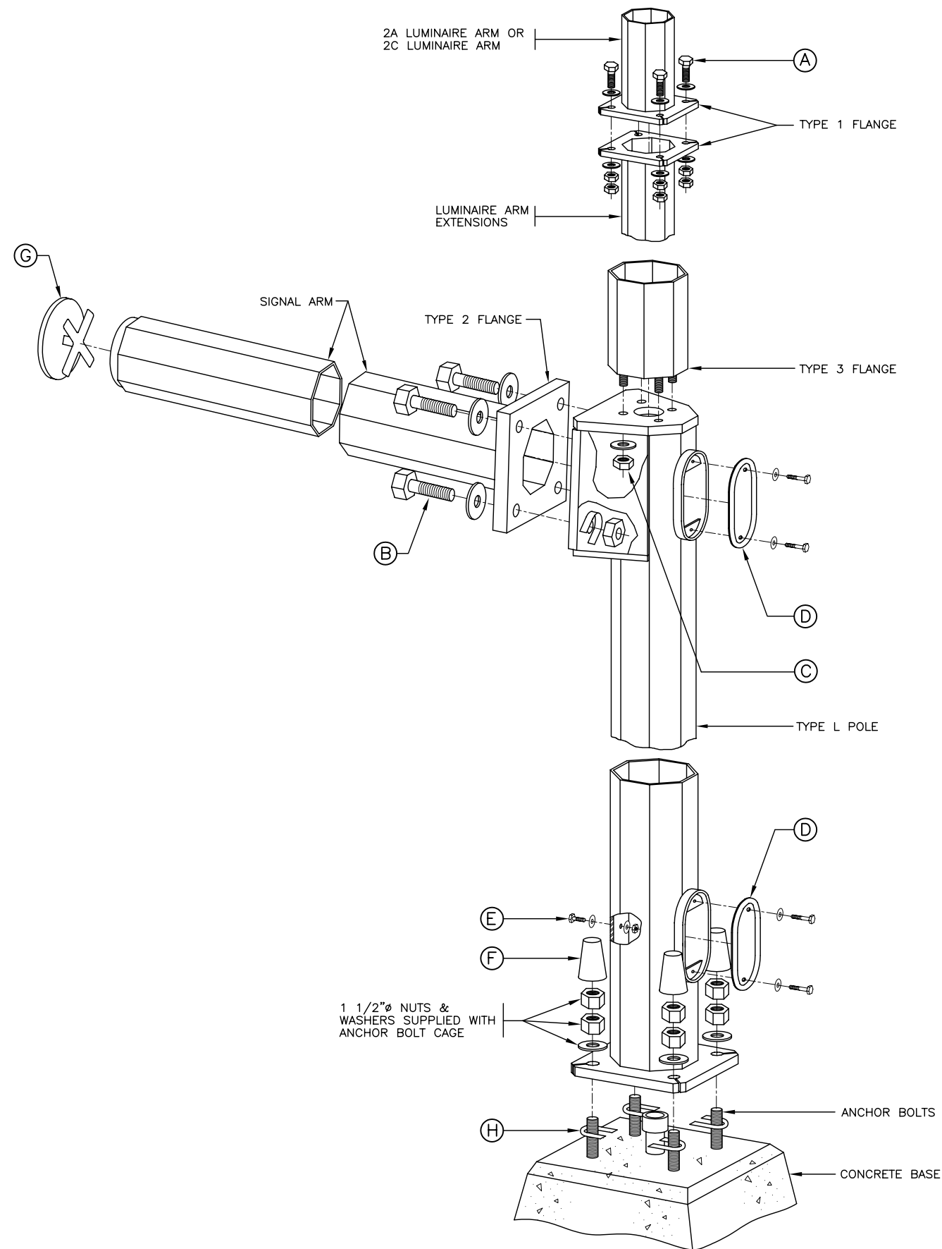
POLE ASSEMBLY DETAIL
