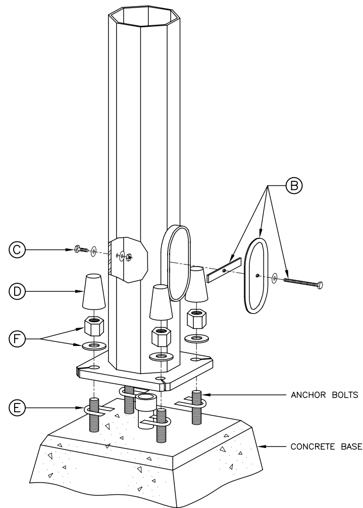
POLE ASSEMBLY DETAIL
