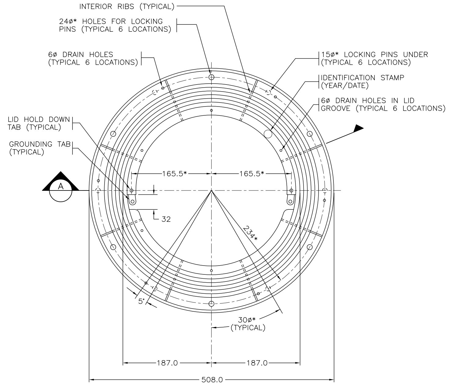
TOP VIEW 1:5
