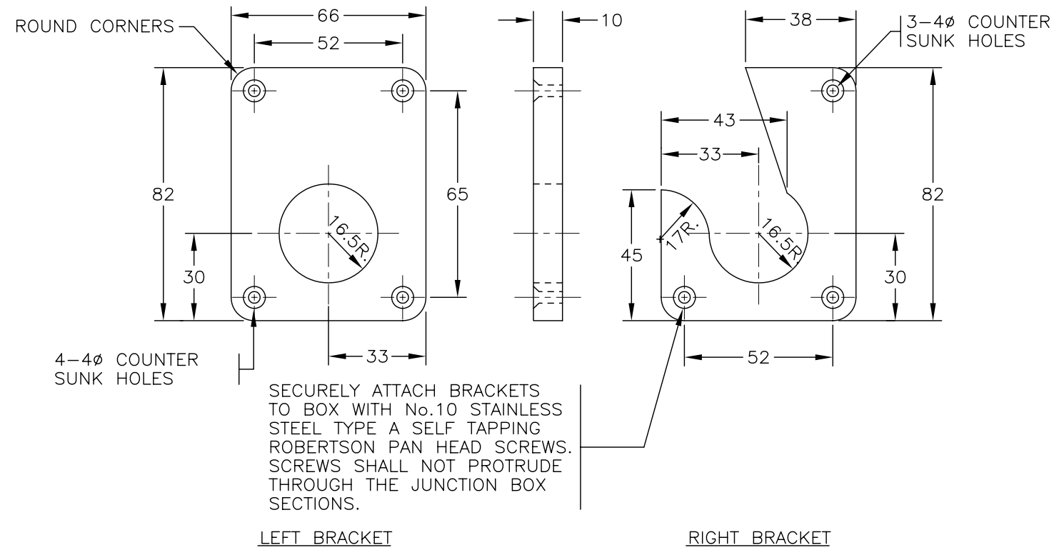
PLASTIC CONDUCTOR SUPPORT BRACKETS
