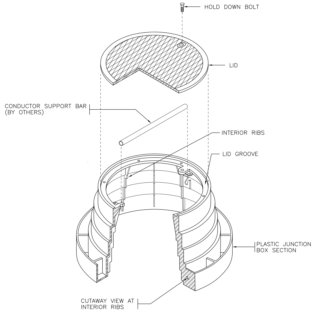
ISOMETRIC CUTAWAY VIEW
