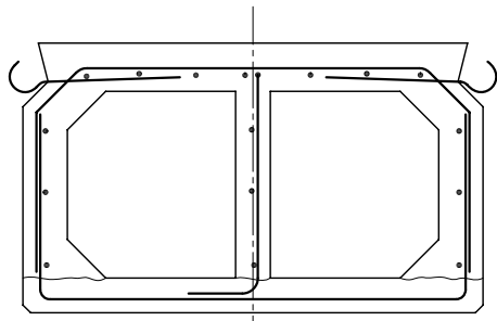
TYPICAL SECTION THROUGH INTERIOR STRINGER SCALE:- 1:10
