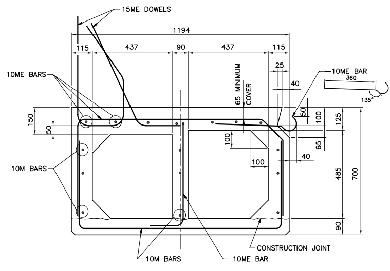
TYPICAL SECTION THROUGH EXTERIOR STRINGER SCALE:- 1:10
