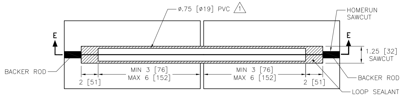
SECTION E-E
