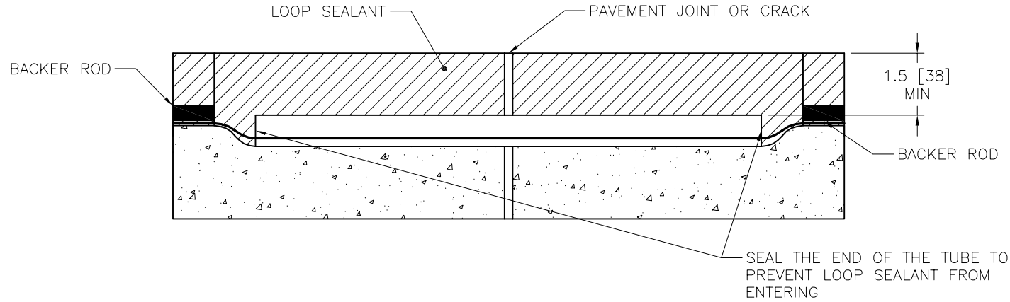
ISOMETRIC SECTION VIEW
