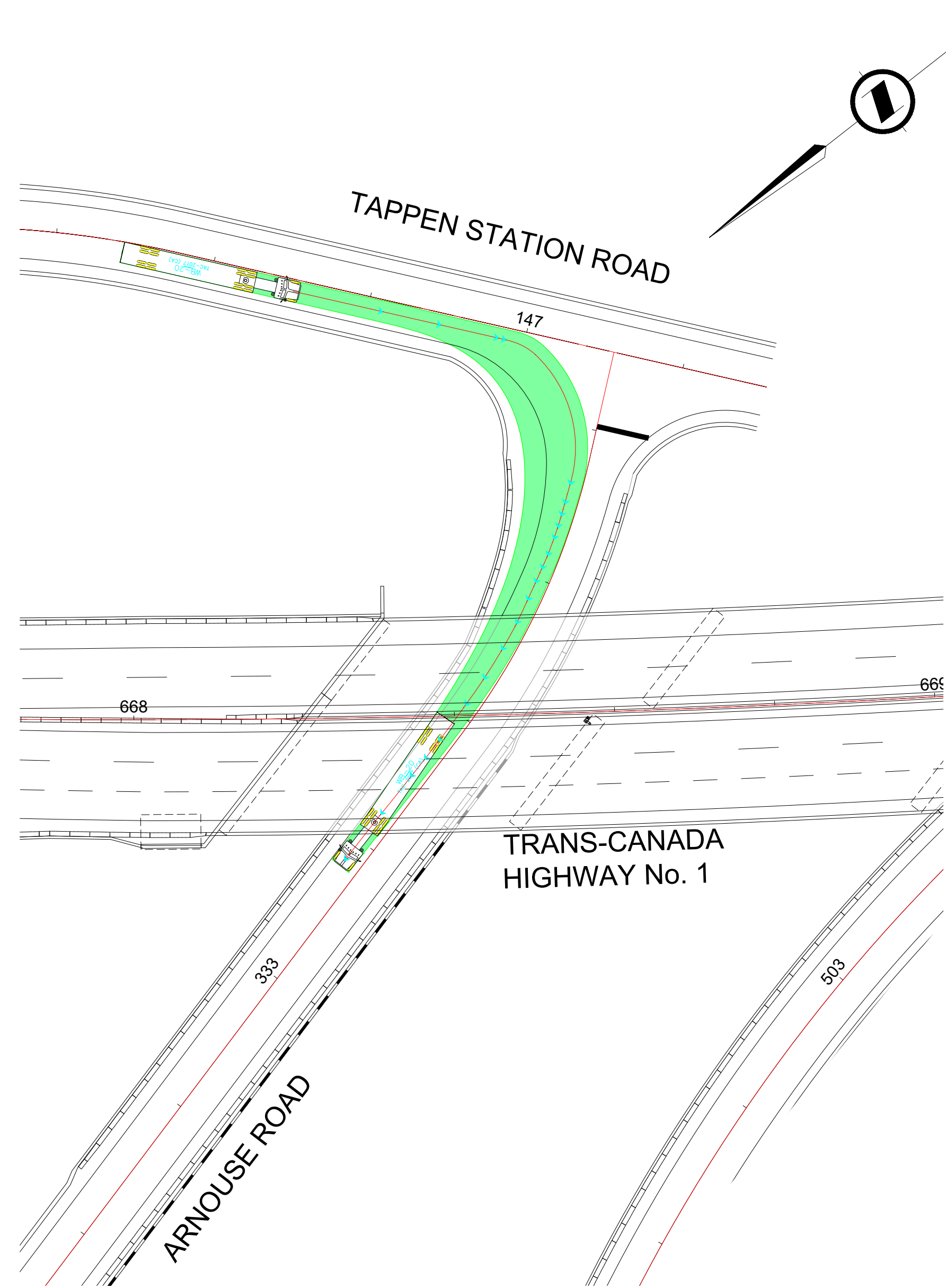
WB-20 TRUCK MOVEMENT ARNOUSE ROAD / TAPPEN STATION ROAD INTERSECTION
