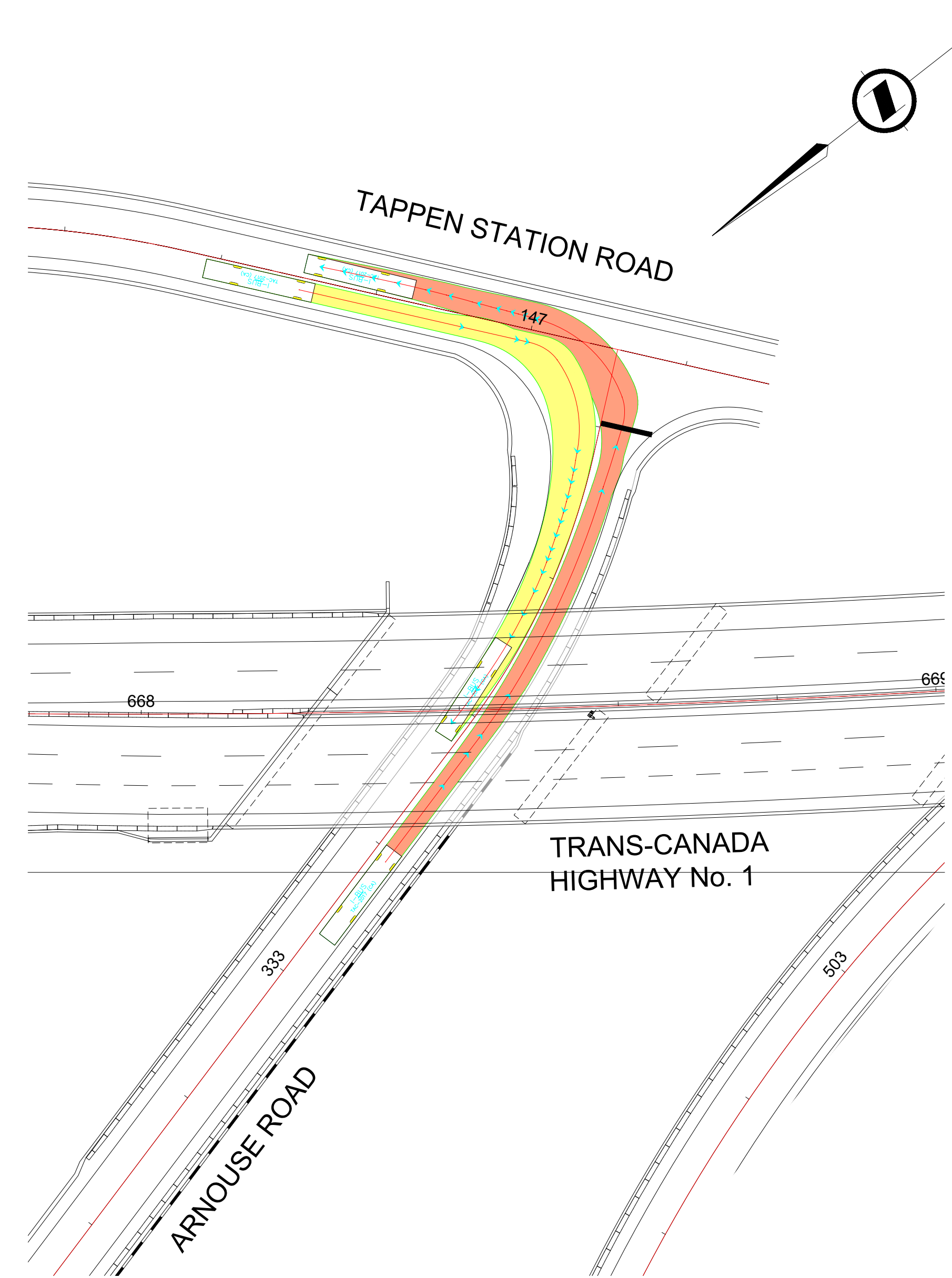
I-BUS TRUCK MOVEMENT ARNOUSE ROAD / TAPPEN STATION ROAD INTERSECTION
