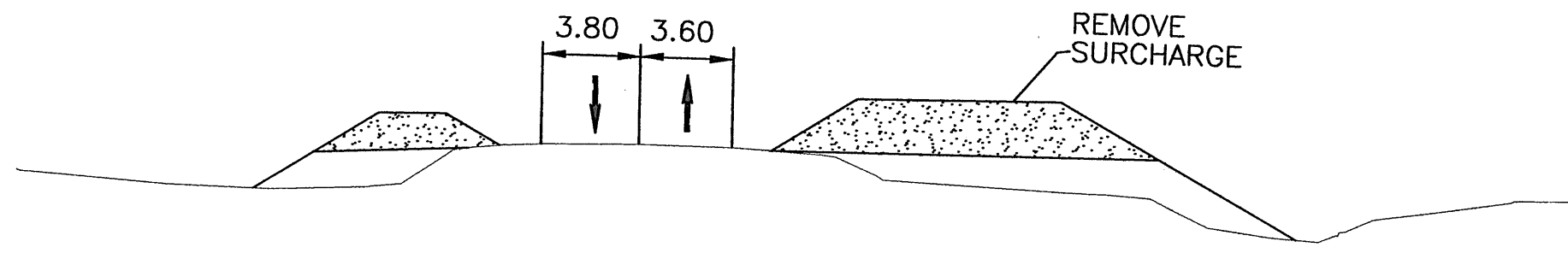
SECTION B-B SCALE 1:250
