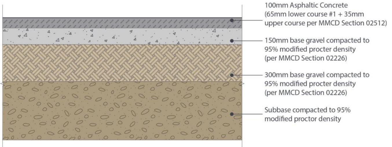
Figure D2 Typical Asphalt Pavement Section
