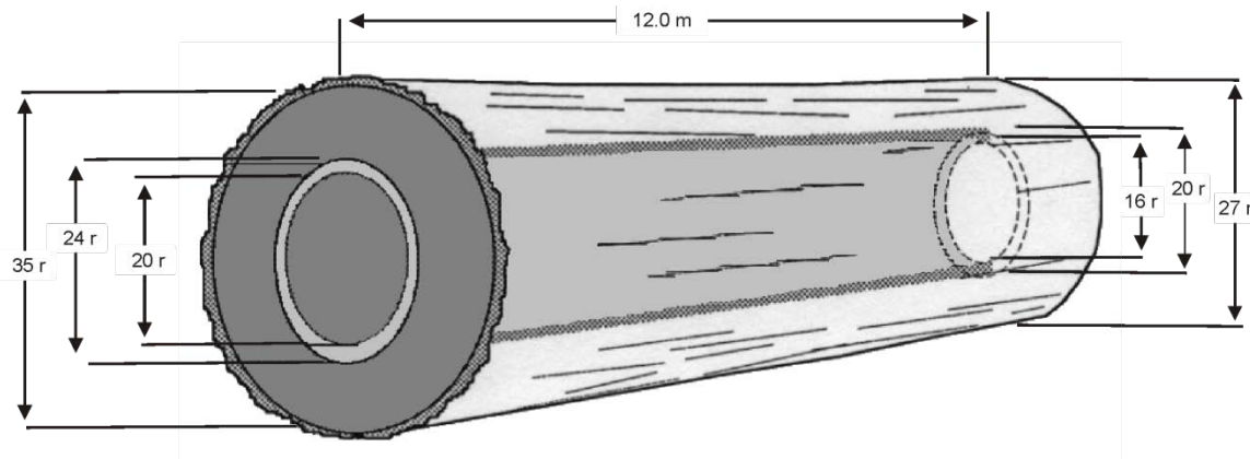
Figure 7.8 A Log with Through-running Ring Rot.
