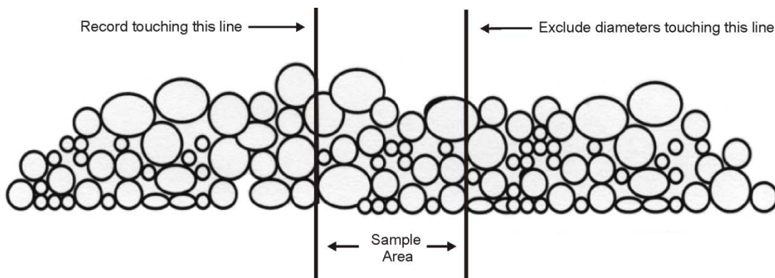
Figure 12.8 Selecting a Sample Section from a Log Deck.
