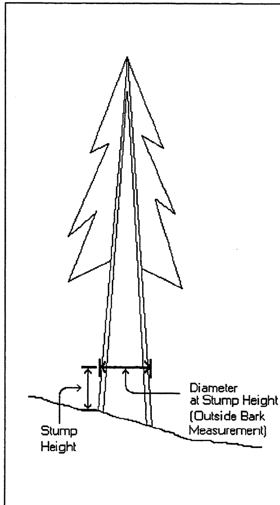
Diagram 1. Felling Specifications
