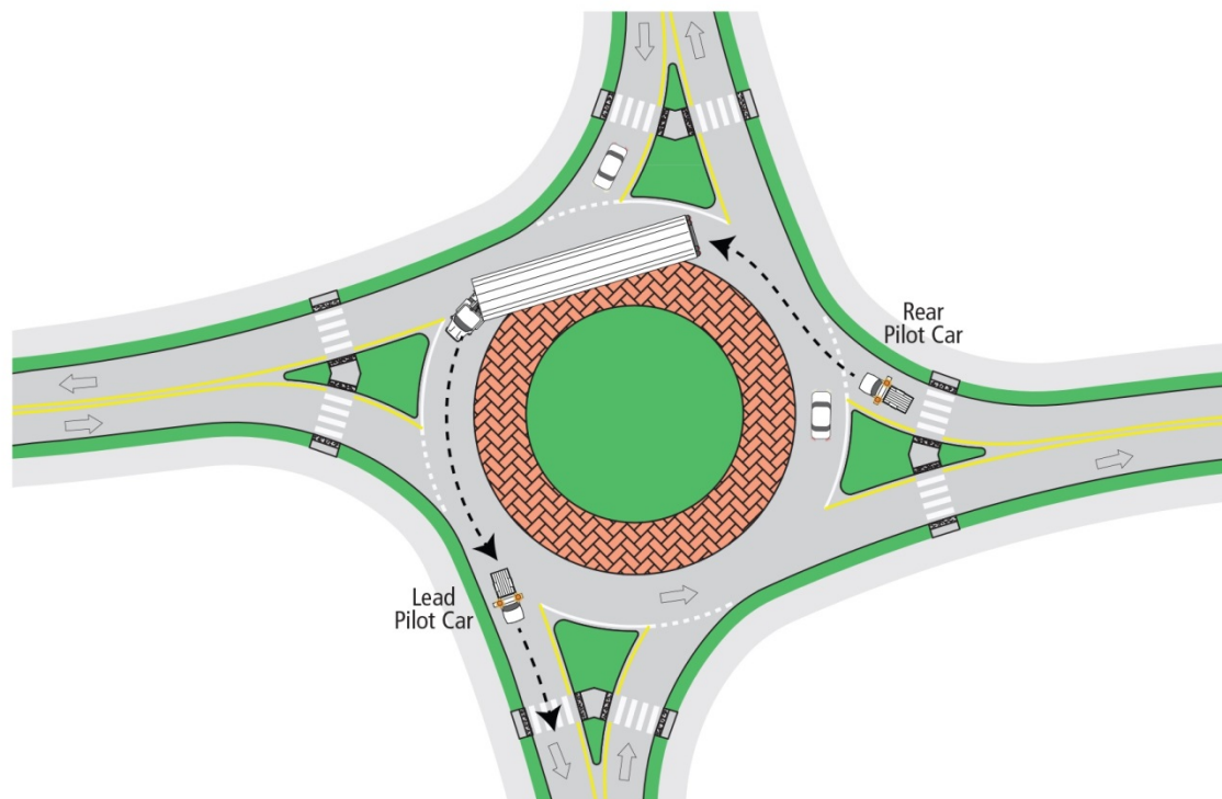
Figure 9.5B Operating through roundabouts – making use of the truck apron
