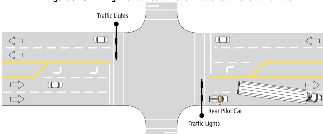
Figure 9.1C Driving in urban conditions – Load returns to travel lane
