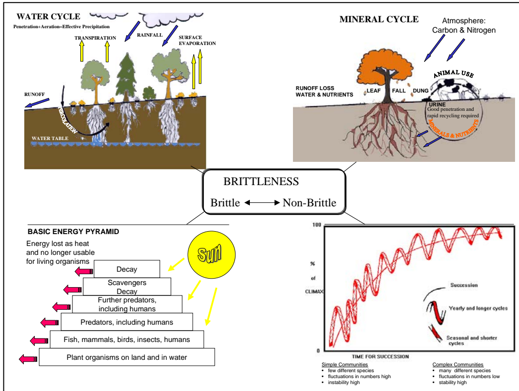
Figure 1 The ecosystem processes functioning in rangelands. Evaluating and monitoring of these processes is the best approach to ecosystem management.
