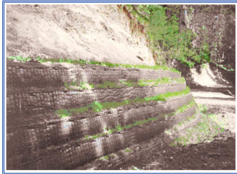
Figure 5 A Reinforced Soil Retaining Wall
