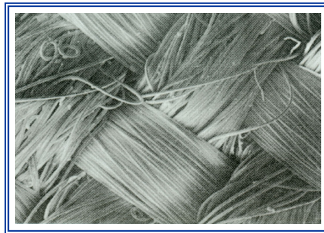
Figure 1 Enlarged Detail of Woven Geotextile
