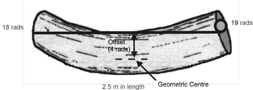
Figure 8.57 Measuring the Offset for 2.5 m Log.
