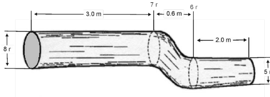
Figure 8.53 Visually Bucking a Log with Crook to Assess Lumber Recovery.
