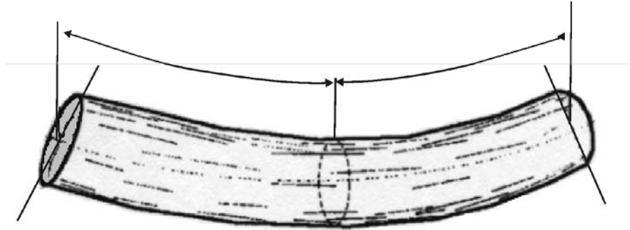
Figure 8.55 Visually Bucking a Log with Sweep to Assess Lumber Recovery.
