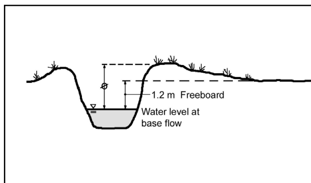
Figure 3 Determining Freeboard
