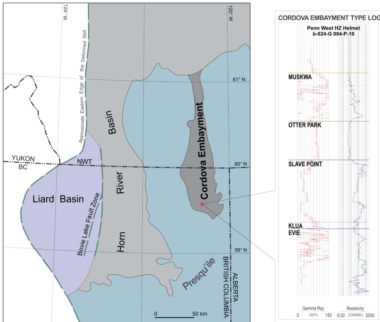
Figure 1. Location of the Cordova Embayment with respect to the Horn River and Liard basins of northeastern British Columbia (outlines of the Liard Basin, Horn River Basin and Cordova Embayment modified from Drees, 1994 and Morrow, 2012). Also shown is the Cordova Embayment Type Log and well location for Penn West HZ Helmet B-024-G-094-P-10.
