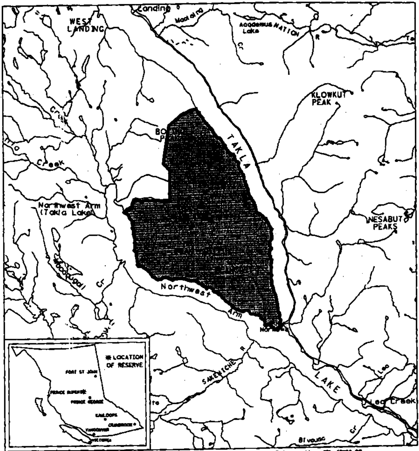
This is a summary sketch of the area shown in black on Mineral Titles Reference Maps (File 12000 09)
