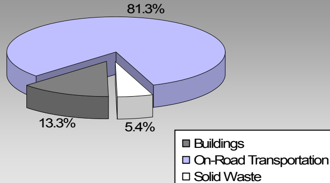
Lions Bay Village 2007 GHG Emissions Sources
