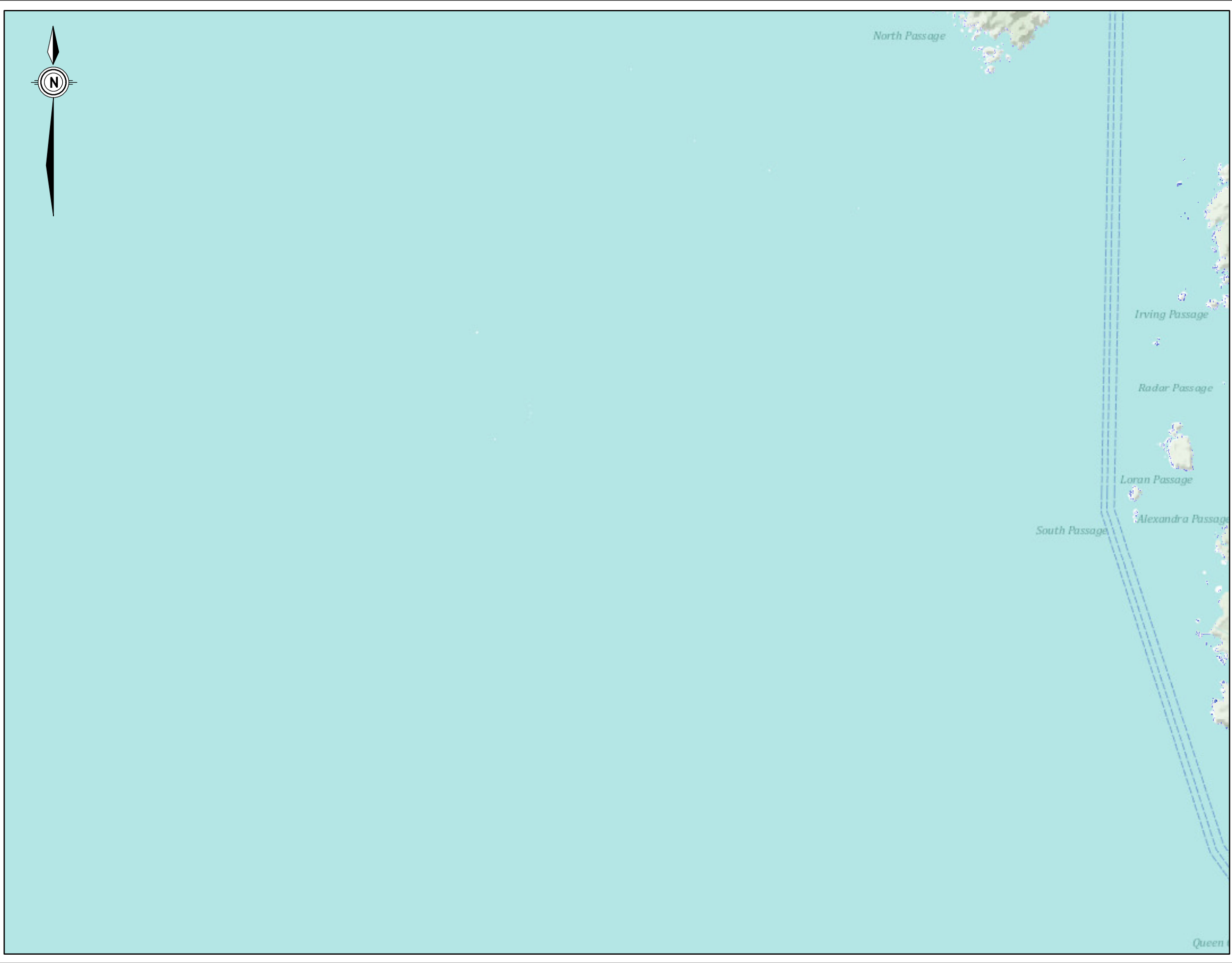
Potential Impact Areas Of Sea Level Rise By The Year 2100 In British Columbia Figure O8
