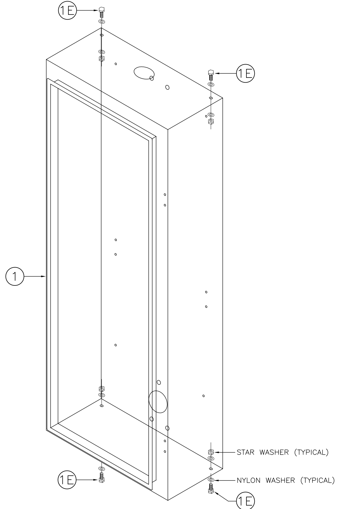
ASSEMBLY VIEW
