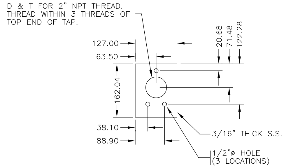
ITEM 1B (LARGE REINFORCING PLATE)
