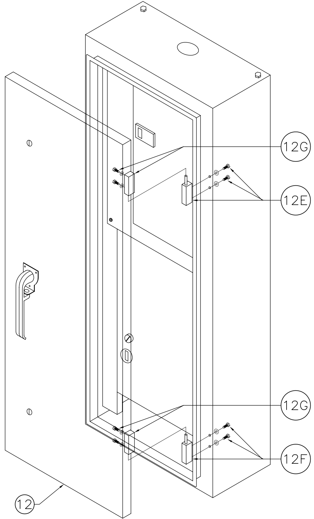
ASSEMBLY VIEW
