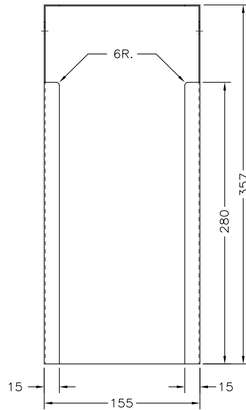
FRONT VIEW 1:4
