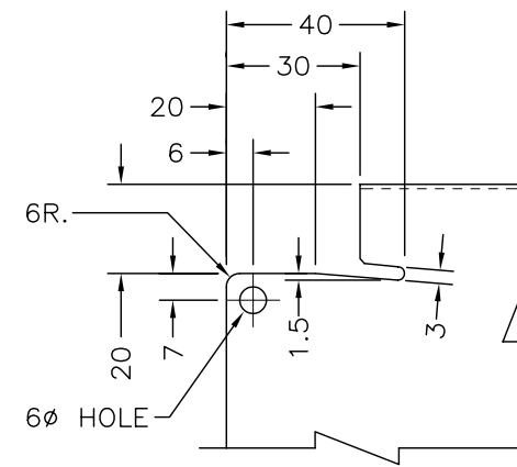
DETAIL A 1:2
