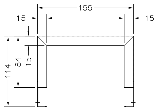
TOP VIEW 1:4
