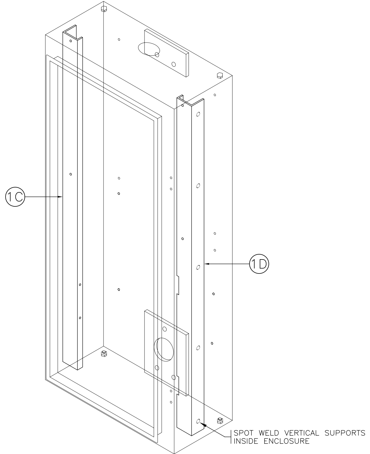
ASSEMBLY VIEW
