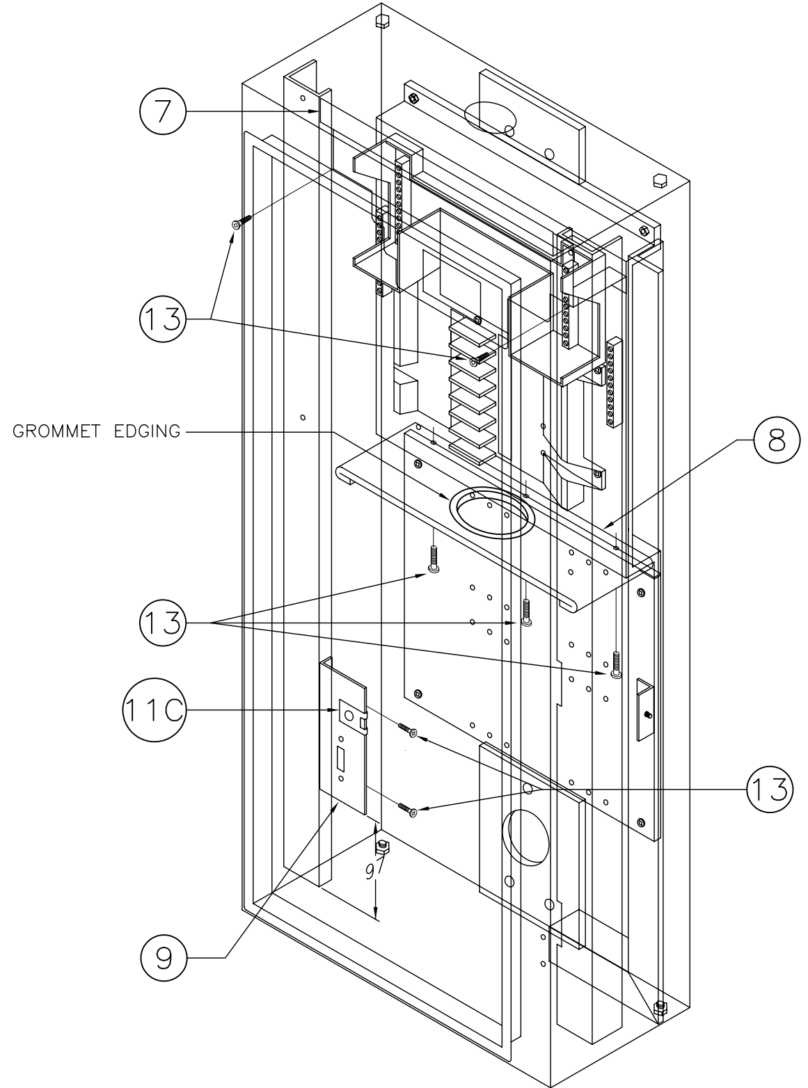
ASSEMBLY VIEW
