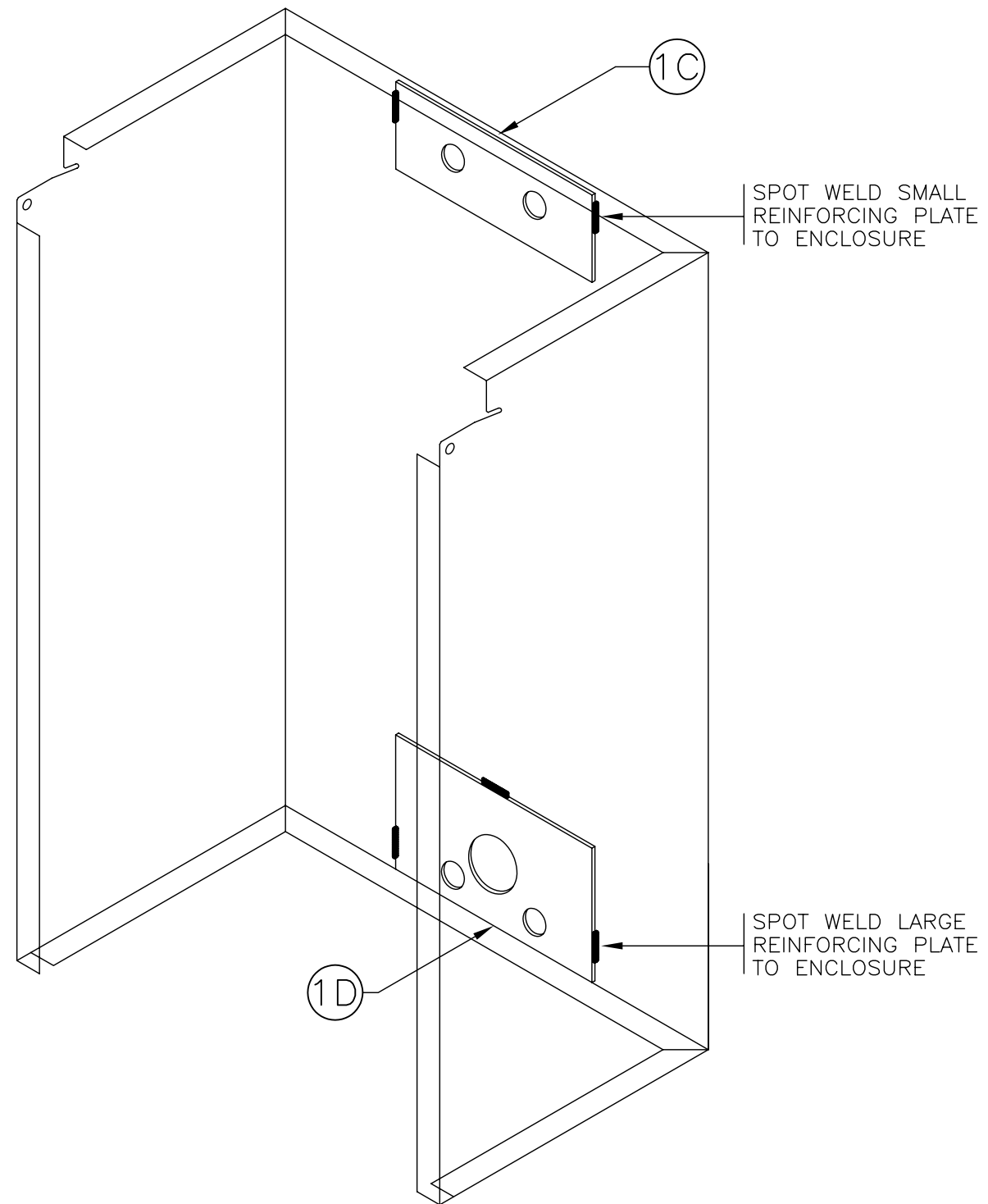
ASSEMBLY VIEW
