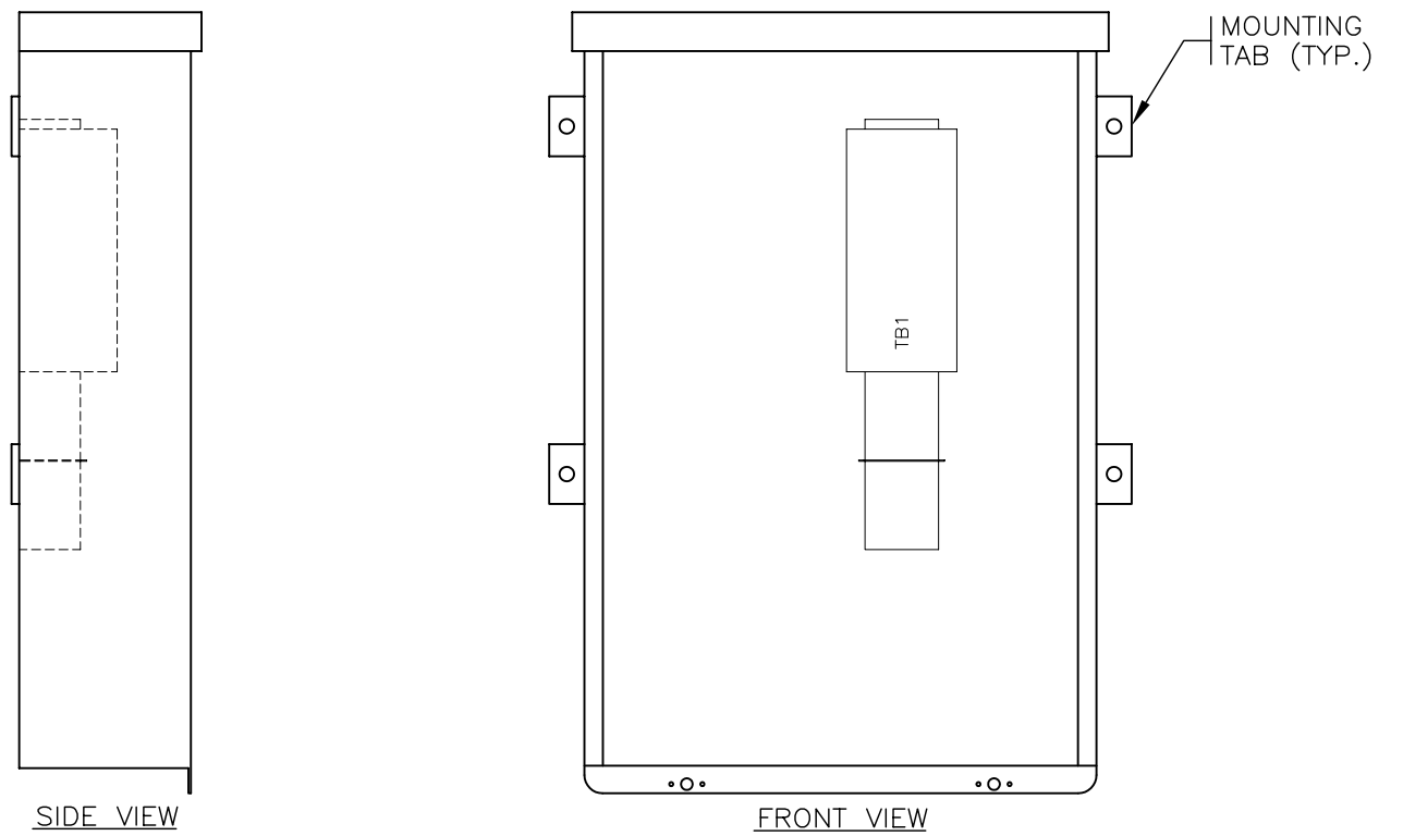
JUNCTION BOX – EQUIPMENT LAYOUT (COVER NOT SHOWN) N.T.S.
