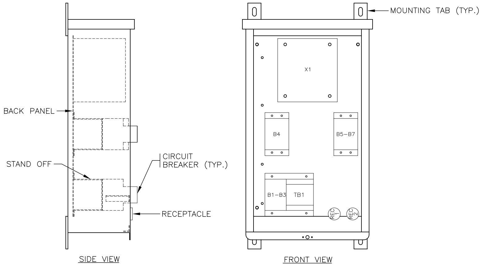
DISTRIBUTION PANEL – EQUIPMENT LAYOUT (COVER NOT SHOWN) N.T.S.
