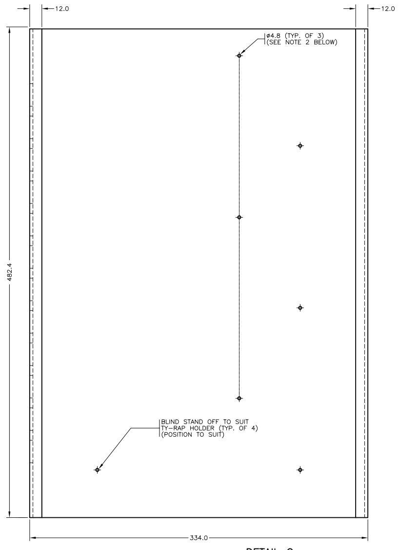
DETAIL C MATERIAL: 1/8" ALUMINIUM SCALE 1:4
