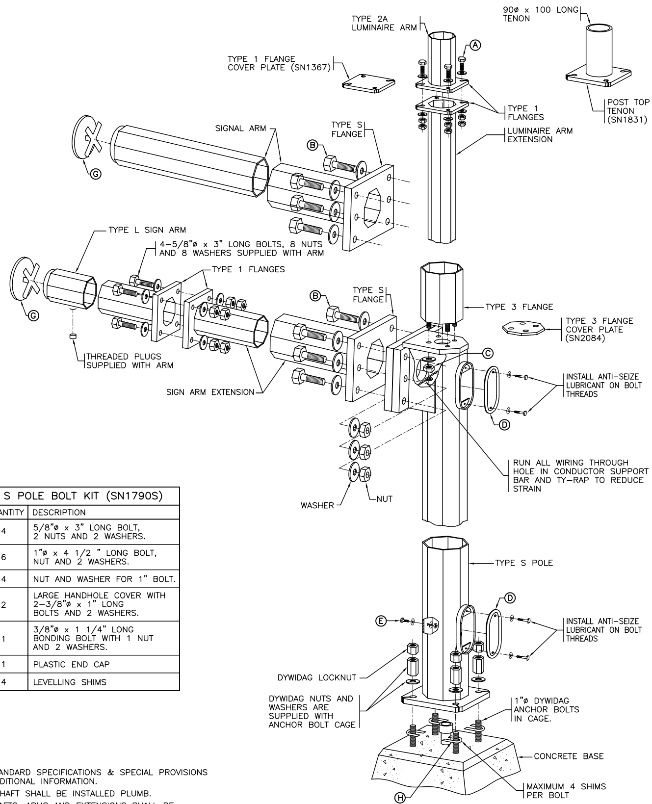
POLE ASSEMBLY DETAIL
