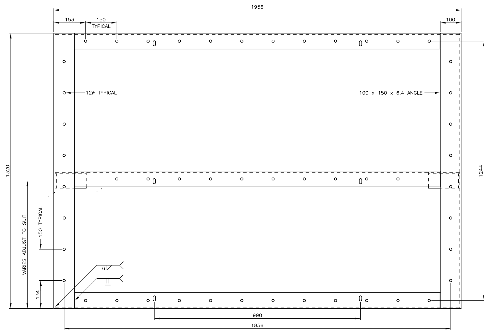
ASSEMBLED FRAME
