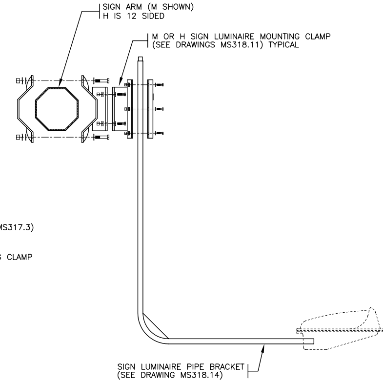
SIGN LUMINAIRE MOUNTING ASSEMBLY VIEW
