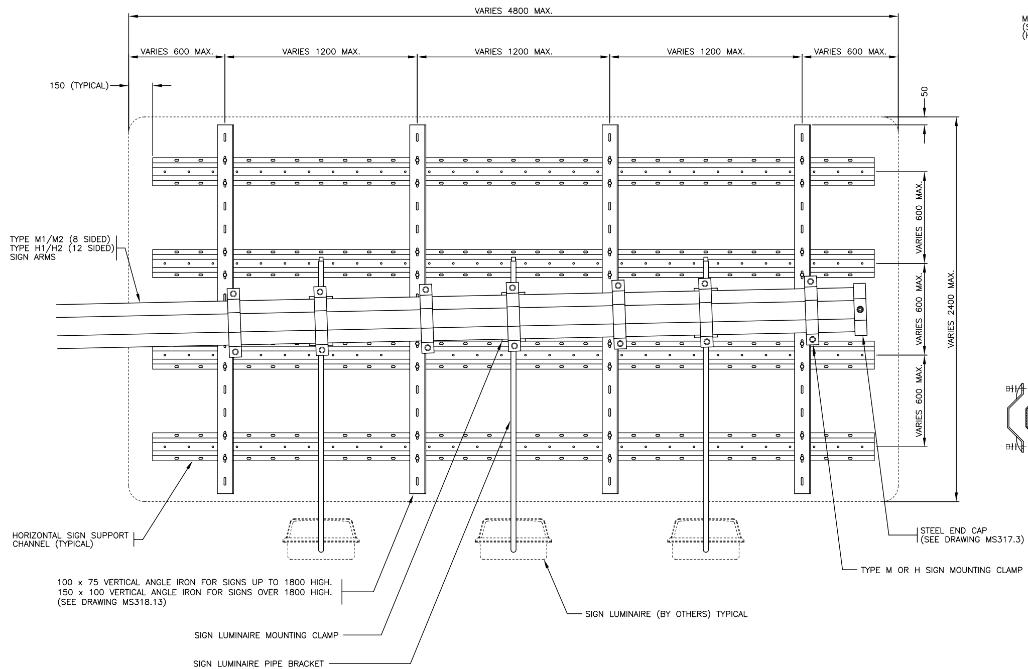
PLYWOOD SIGN AND SIGN LUMINAIRE MOUNTING DETAILS – REAR VIEW
