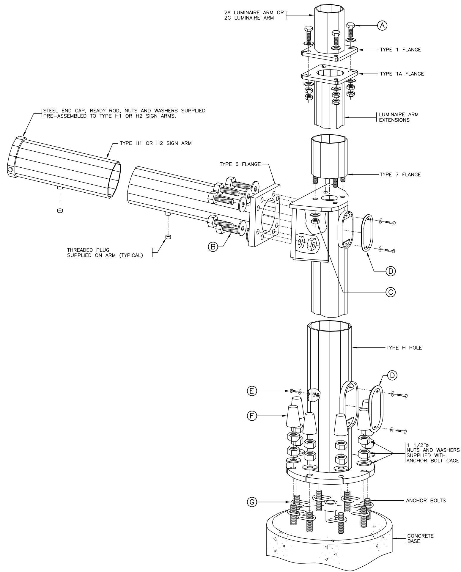
POLE ASSEMBLY DETAIL
