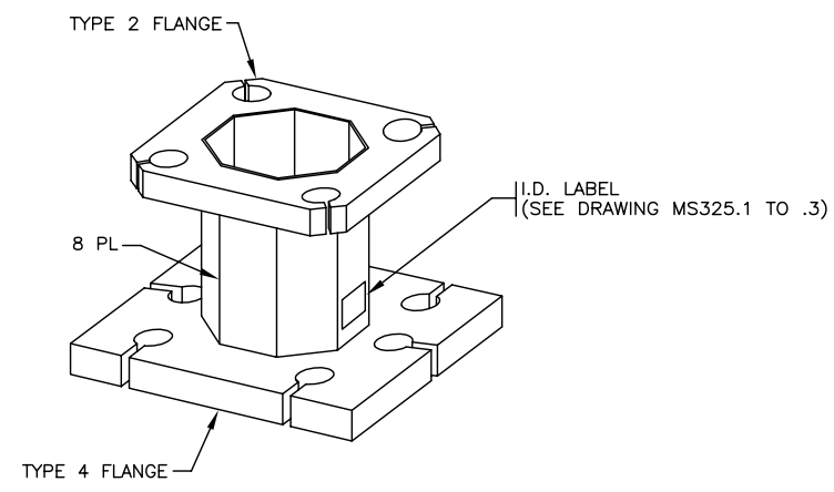
TYPE 4 TO TYPE 2 FLANGE ADAPTOR
