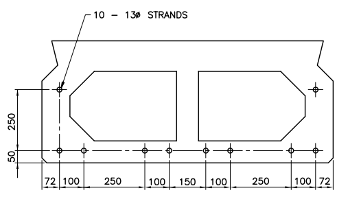
PRESTRESSING STRAND LAYOUT SCALE:- 1:10
