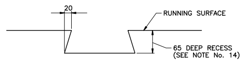
LIFTING DEVICE RECESS DETAIL SCALE:- 1:5
