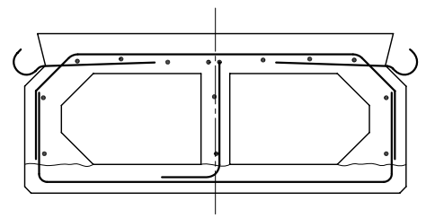
TYPICAL SECTION THROUGH INTERIOR STRINGER SCALE:- 1:10
